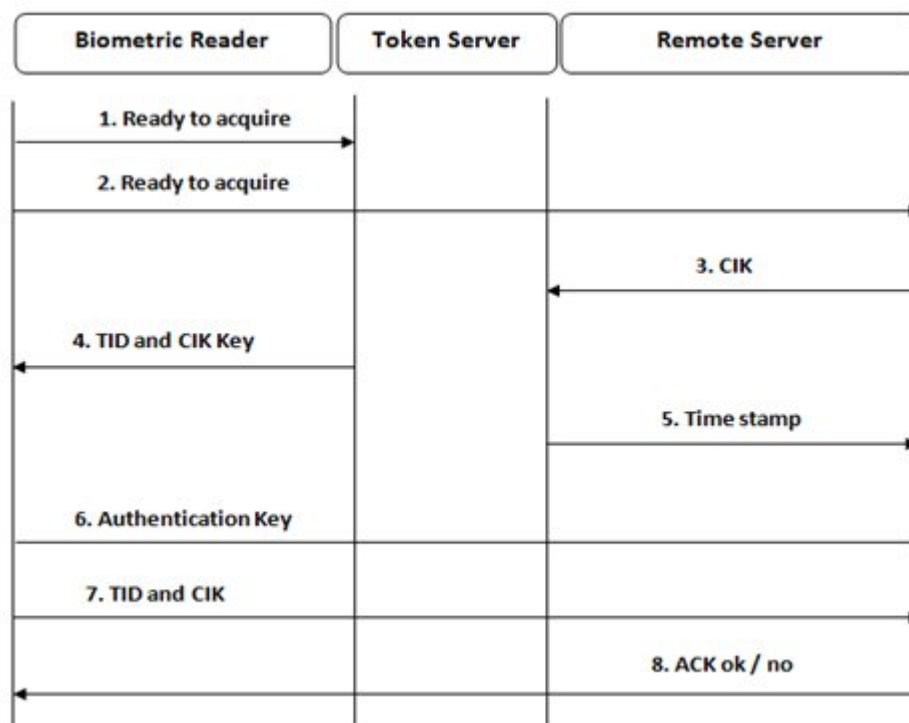
Figure 18. A trusted third party based secure network transaction
