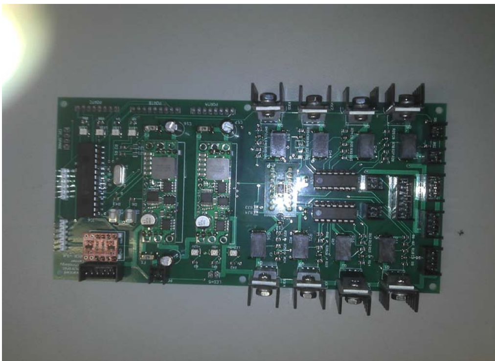
Fig. 24. Main control board of stationery contactless fingerprinting system
