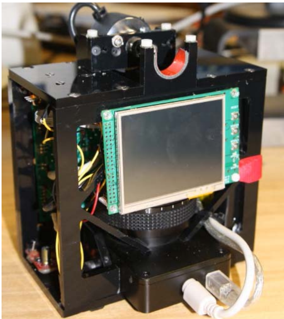
Fig. 26 Contactless fingerprinting with area camera. Finger rotates
