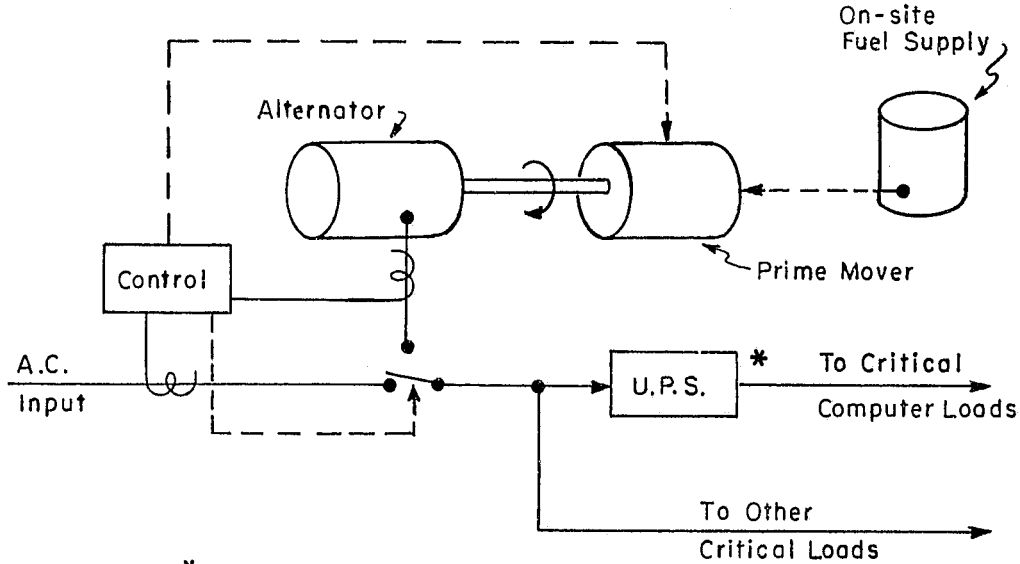
FIGURE 10. UPS with on-site generation.
