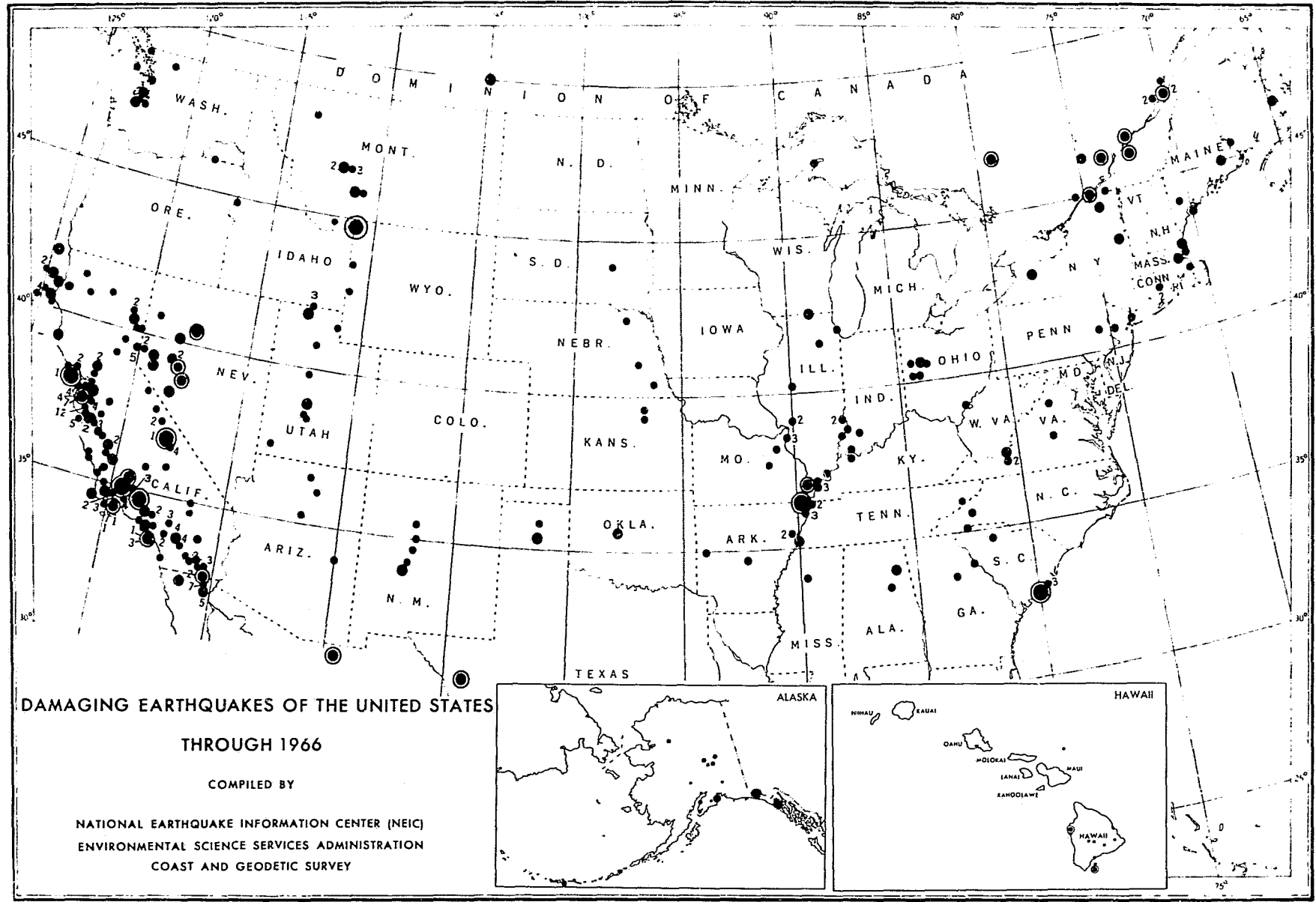
FIGURE 2. Damaging earthquakes of the United States through 1966.
