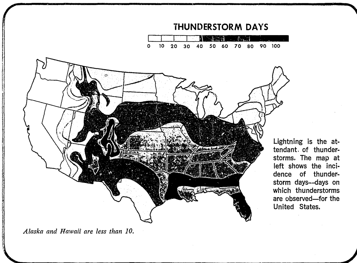
FIGURE 5. Thunderstorm days.
