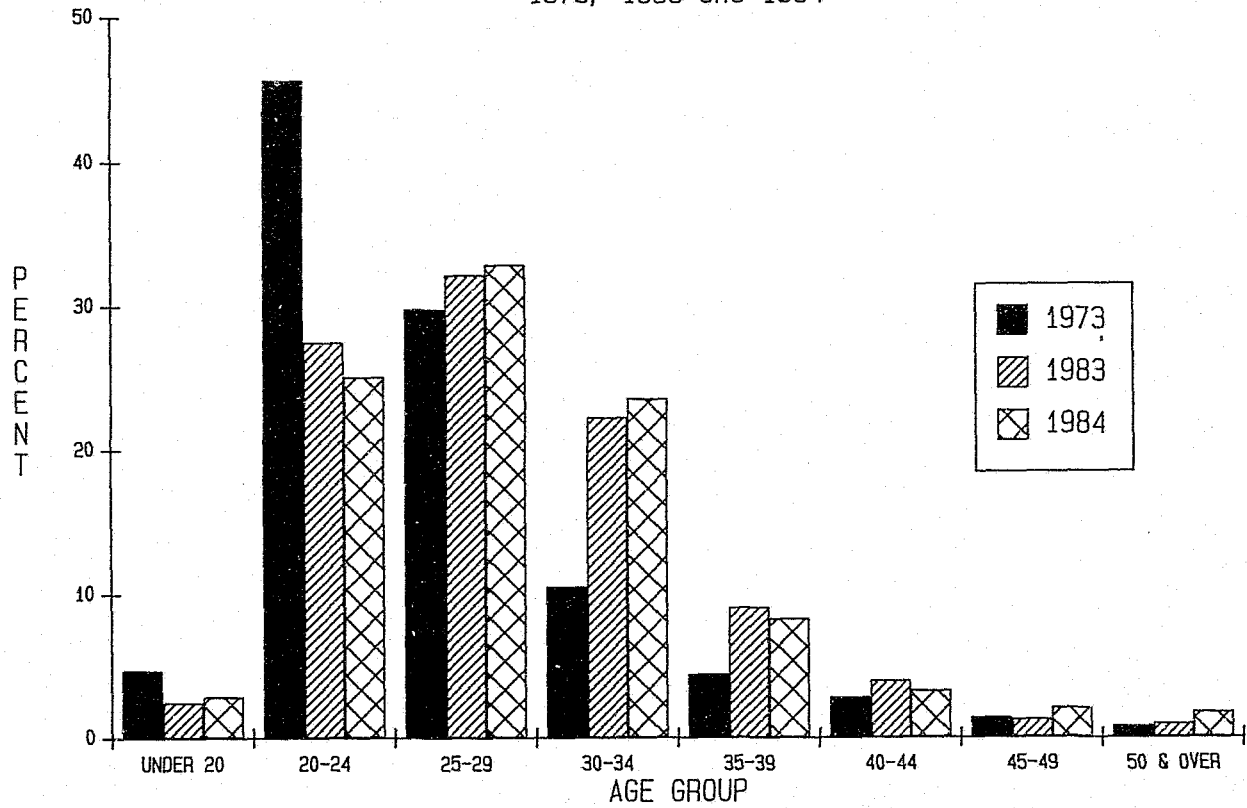
CHART XIV A AGE AT ADMISSION Male Civil Narcotic Addicts Newly Received From Court 1973, 1983 and 1984
