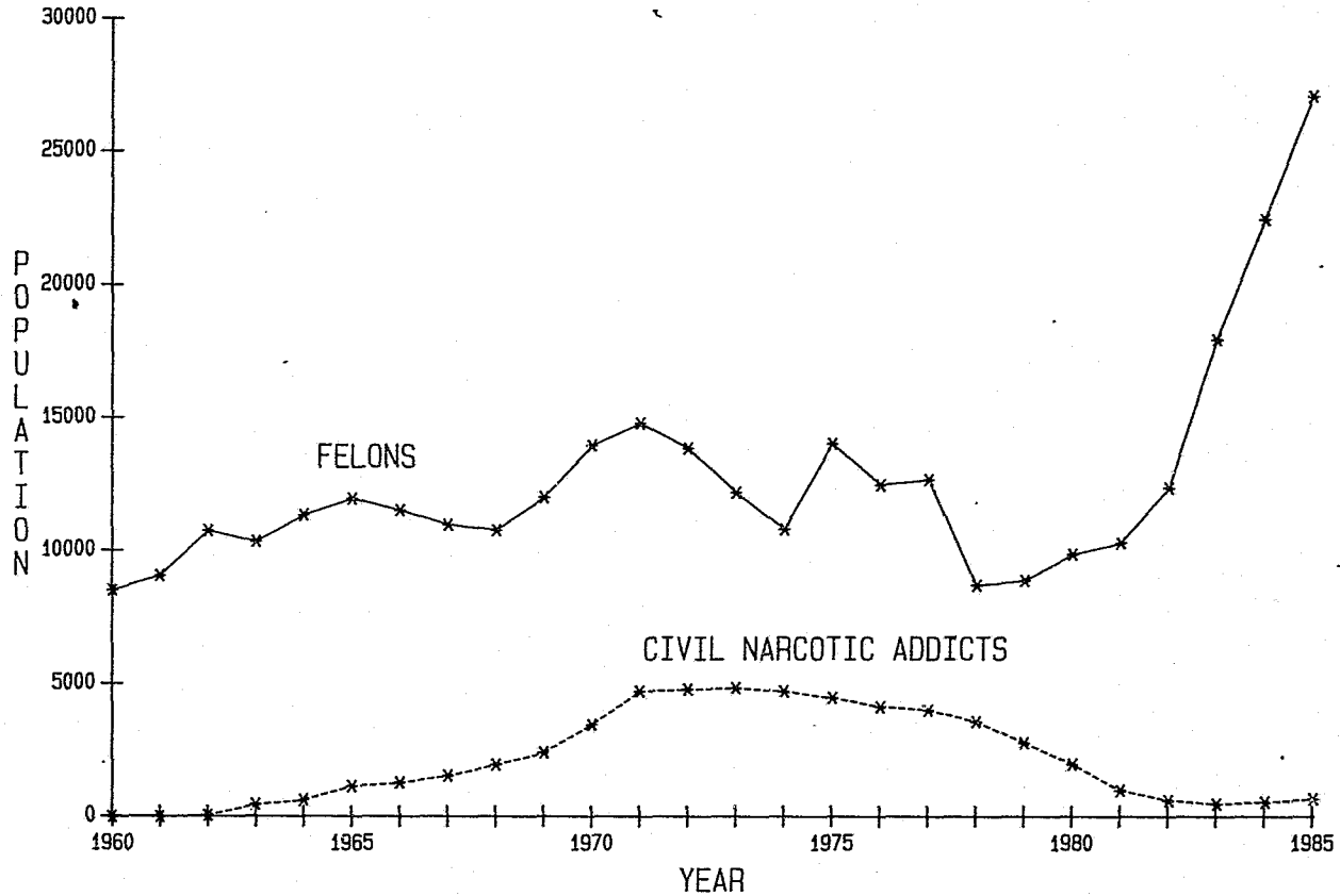
CHART X A MALE PAROLE AND OUTPATIENT POPULATION DECEMBER 31, 1960 THROUGH 1985
