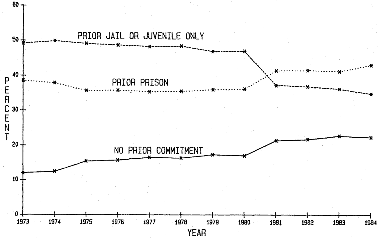
CHART VII A PRIOR COMMITMENT RECORD Percentage Distribution of Male Felons in Prison December 31, 1973 through 1984
