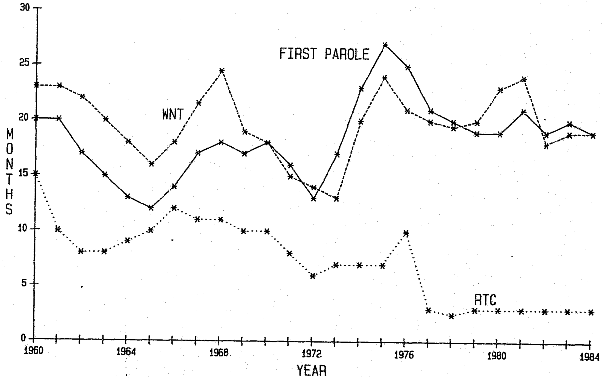
CHART IX B TYPE OF PAROLE AND MEDIAN TIME SERVED IN PRISON BEFORE LAST PAROLE FEMALE FELONS 1960 THROUGH 1984
