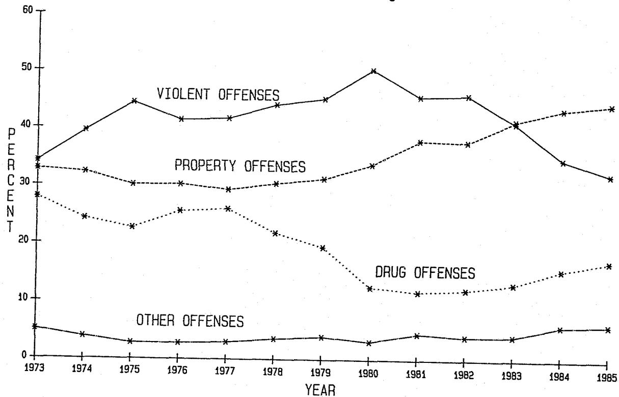
CHART V B OFFENSE GROUPS Percentage Distribution of Female Felons in Prison December 31, 1973 through 1985
