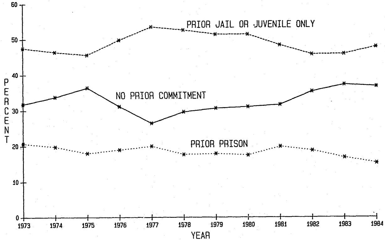
CHART VII B PRIOR COMMITMENT RECORD PERCENTAGE DISTRIBUTION OF FEMALE FELONS IN PRISON DECEMBER 31, 1973 THROUGH 1984
