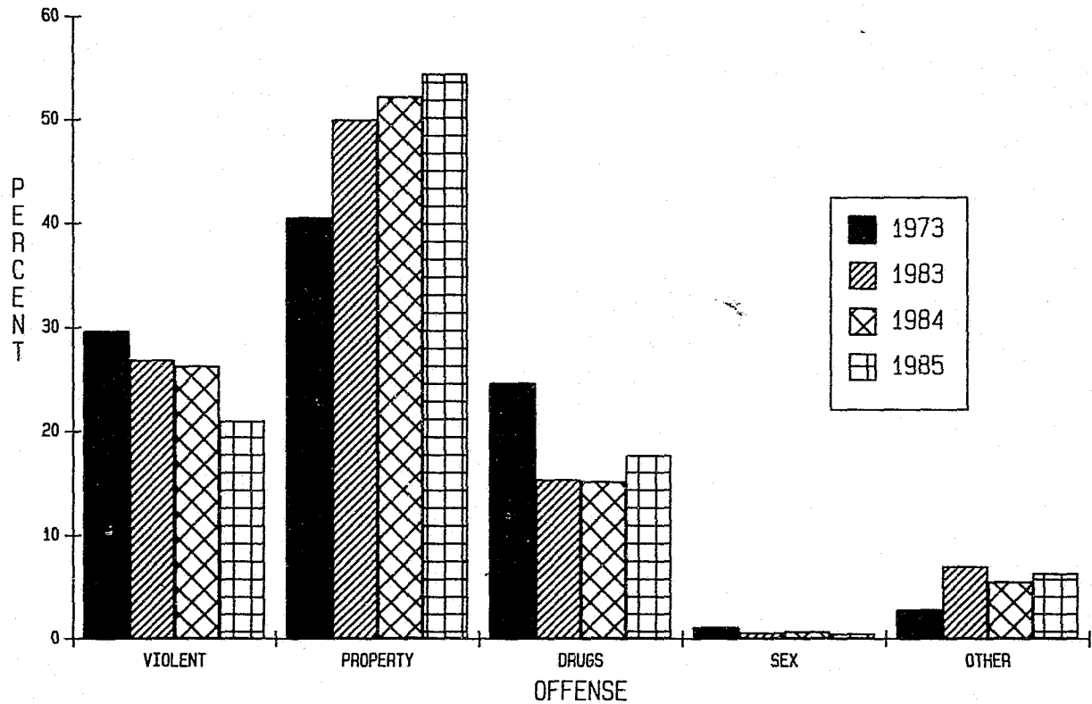
CHART XI B OFFENSE GROUPS Percentage Distribution of Female Felons on Parole December 31, 1973, 1983, 1984 and 1985
