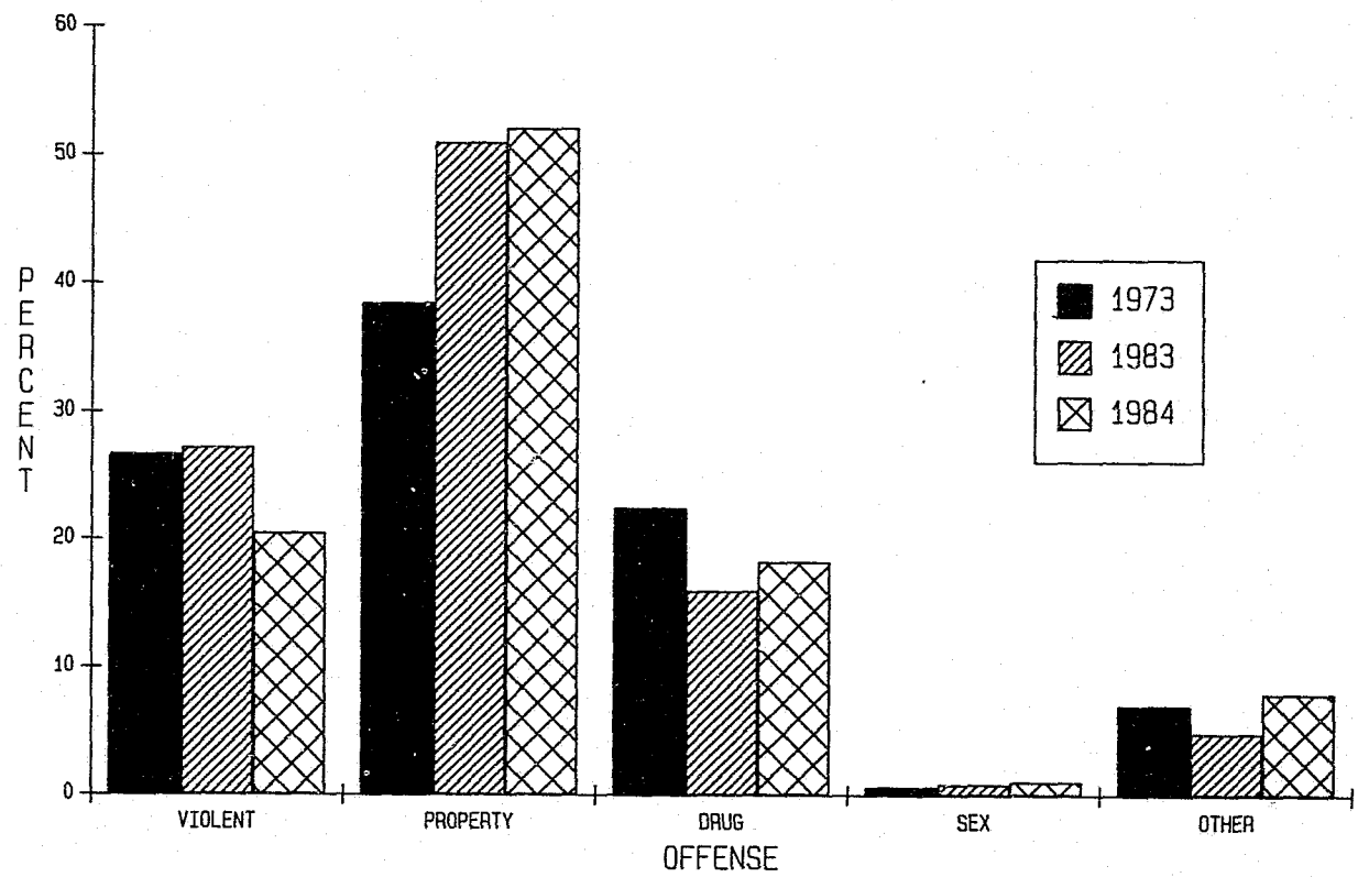
CHART II B OFFENSE GROUPS EXPRESSED IN PERCENTAGES Female Felons Newly Received From Court 1973, 1983 and 1984
