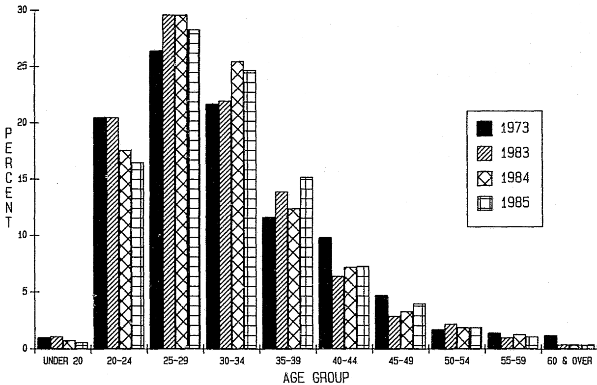
CHART VI B AGE GROUP Percentage Distribution of Female Felons in Prison December 31, 1973, 1983, 1984 and 1985
