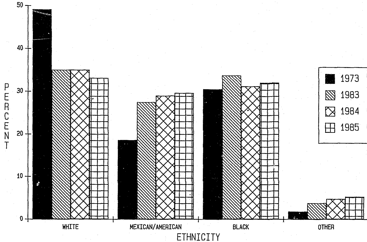
CHART IV A RACIAL-ETHNIC GROUP Male Felons Newly Received From Court 1973, 1983, 1984 and 1985
