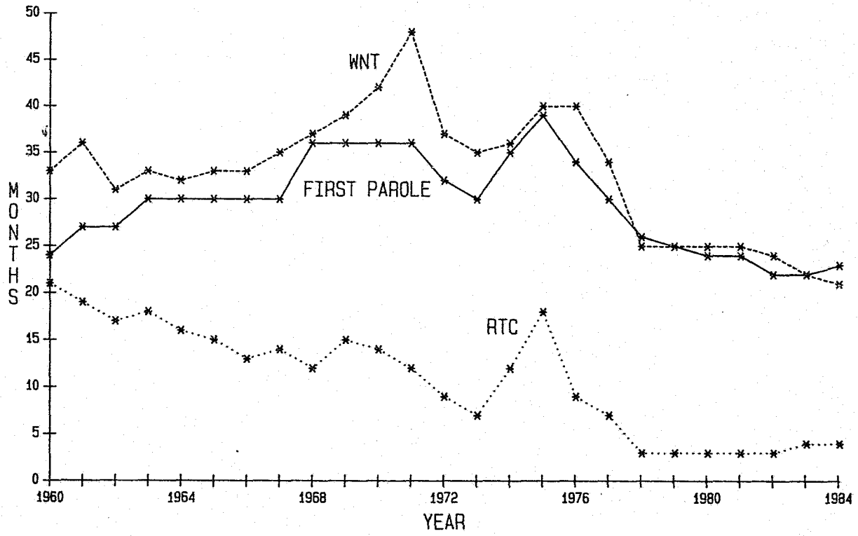
CHART IX A TYPE OF PAROLE AND MEDIAN TIME SERVED IN PRISON BEFORE LAST PAROLE MALE FELONS 1960 THROUGH 1984
