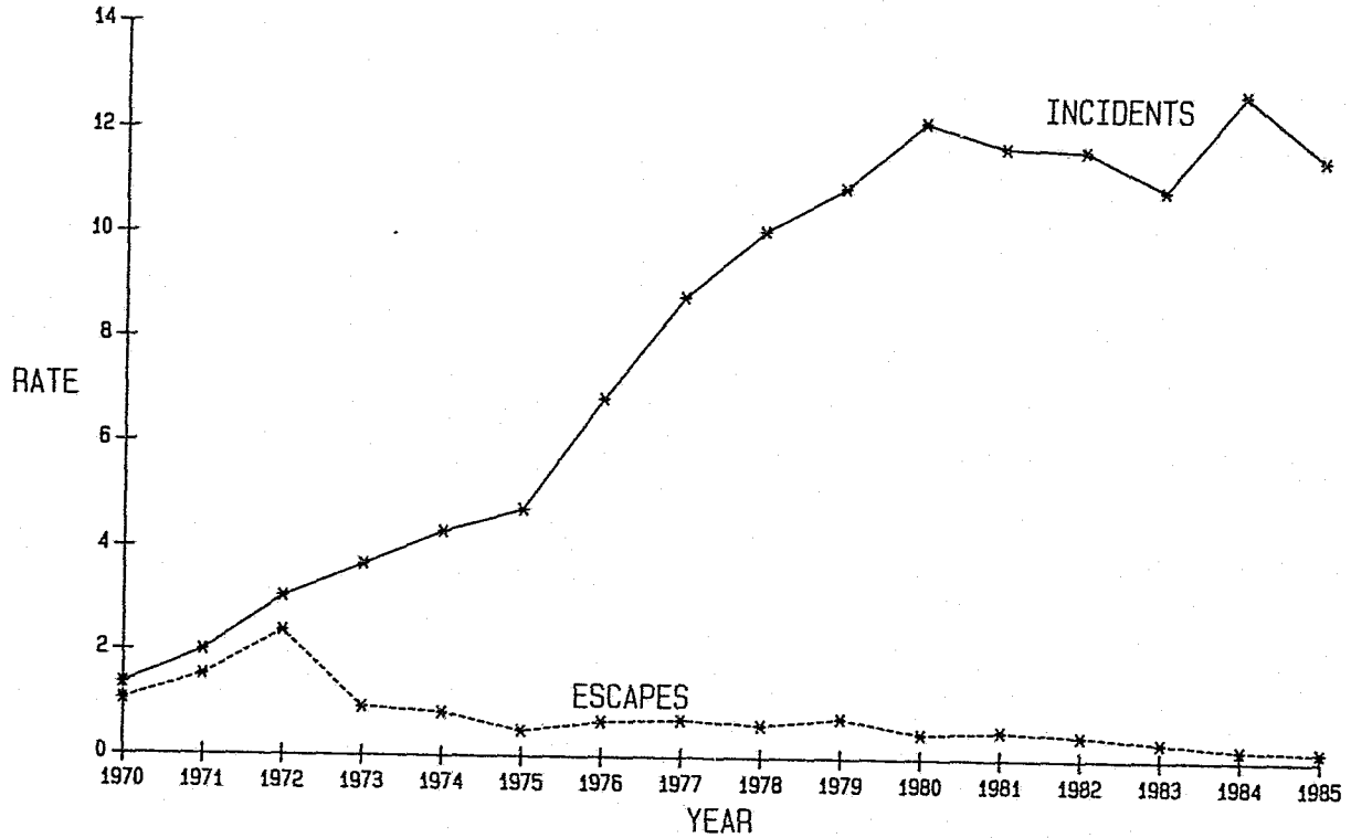
CHART VIII RATE PER 100 AVERAGE DAILY POPULATION OF INCIDENTS AND ESCAPES FROM INSTITUTIONS 1970 THROUGH 1985
