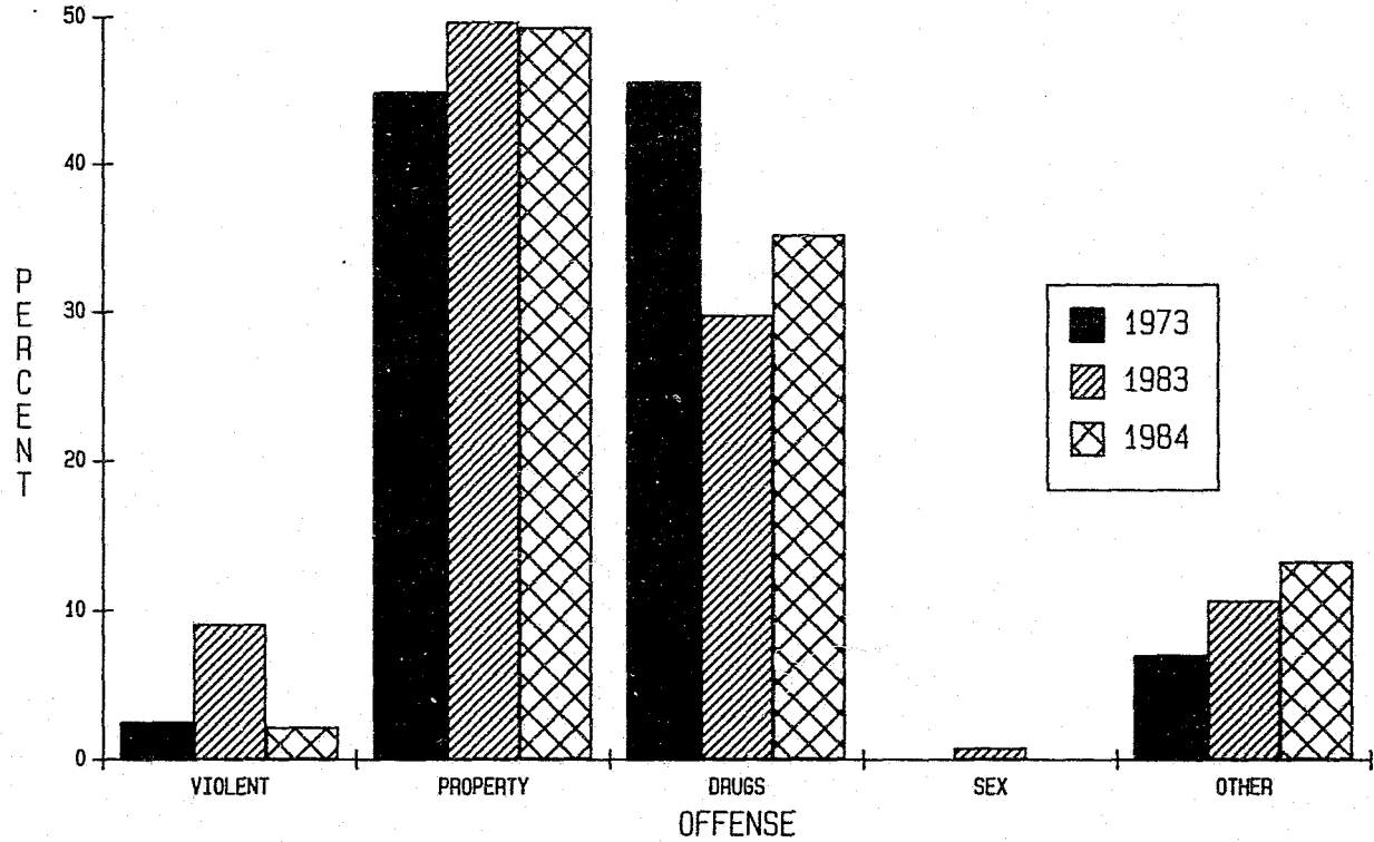
CHART XII B OFFENSE GROUPS Female Civil Narcotic Addicts Newly Received From Court December 31, 1973, 1983 and 1984
