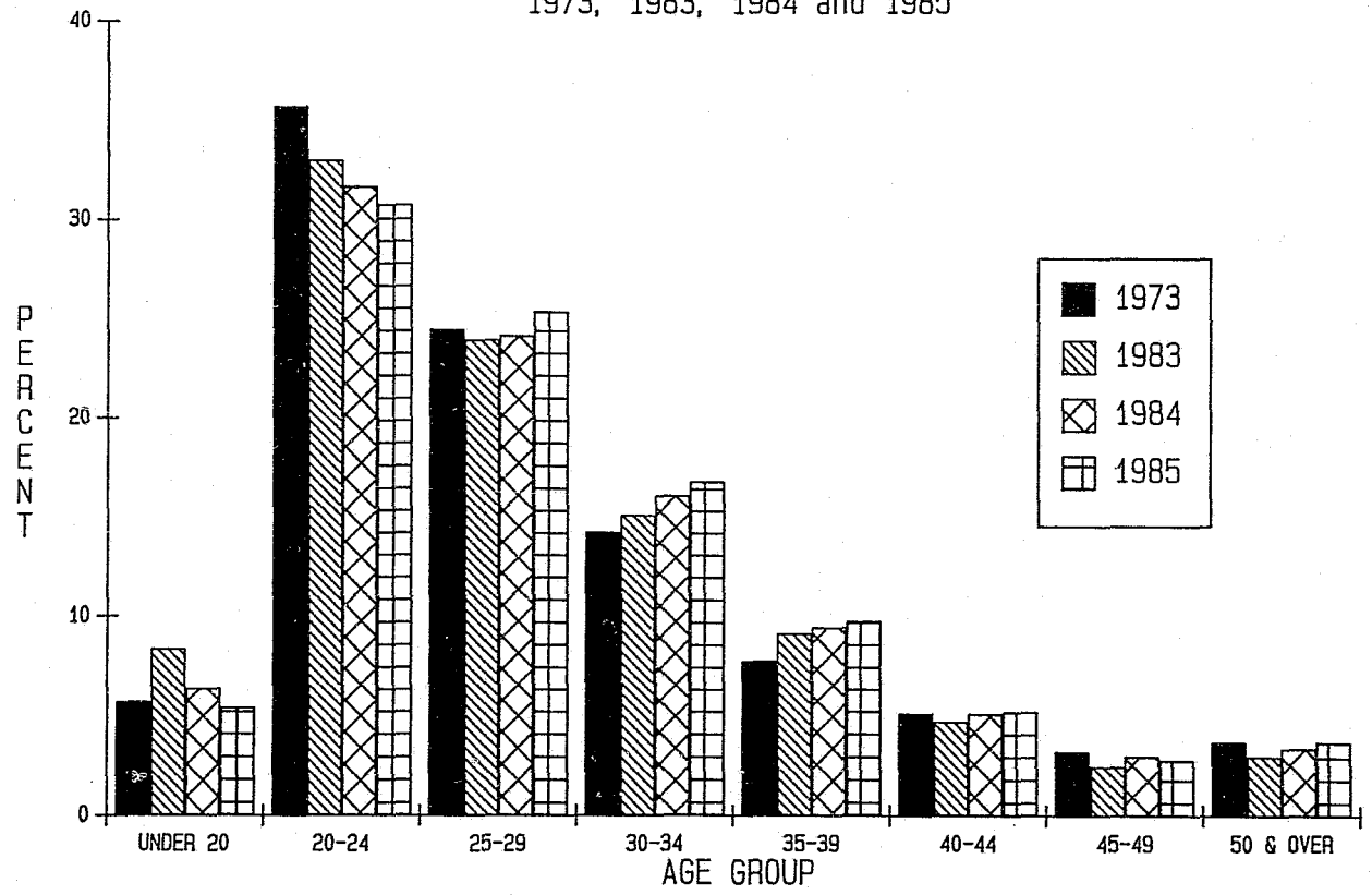
CHART III A AGE AT ADMISSION Male Felons Newly Received From Court 1973, 1983, 1984 and 1985
