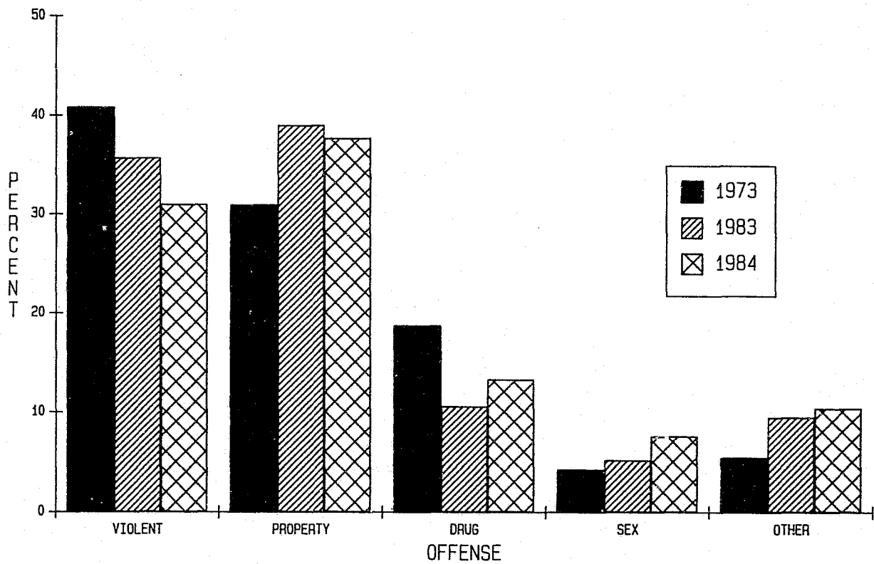
CHART II A OFFENSE GROUPS EXPRESSED IN PERCENTAGES Male Felons Newly Received From Court 1973, 1983 and 1984
