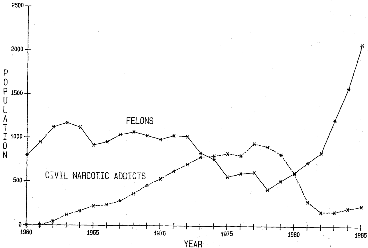
CHART X B FEMALE PAROLE AND OUTPATIENT POPULATION DECEMBER 31, 1960 THROUGH 1985
