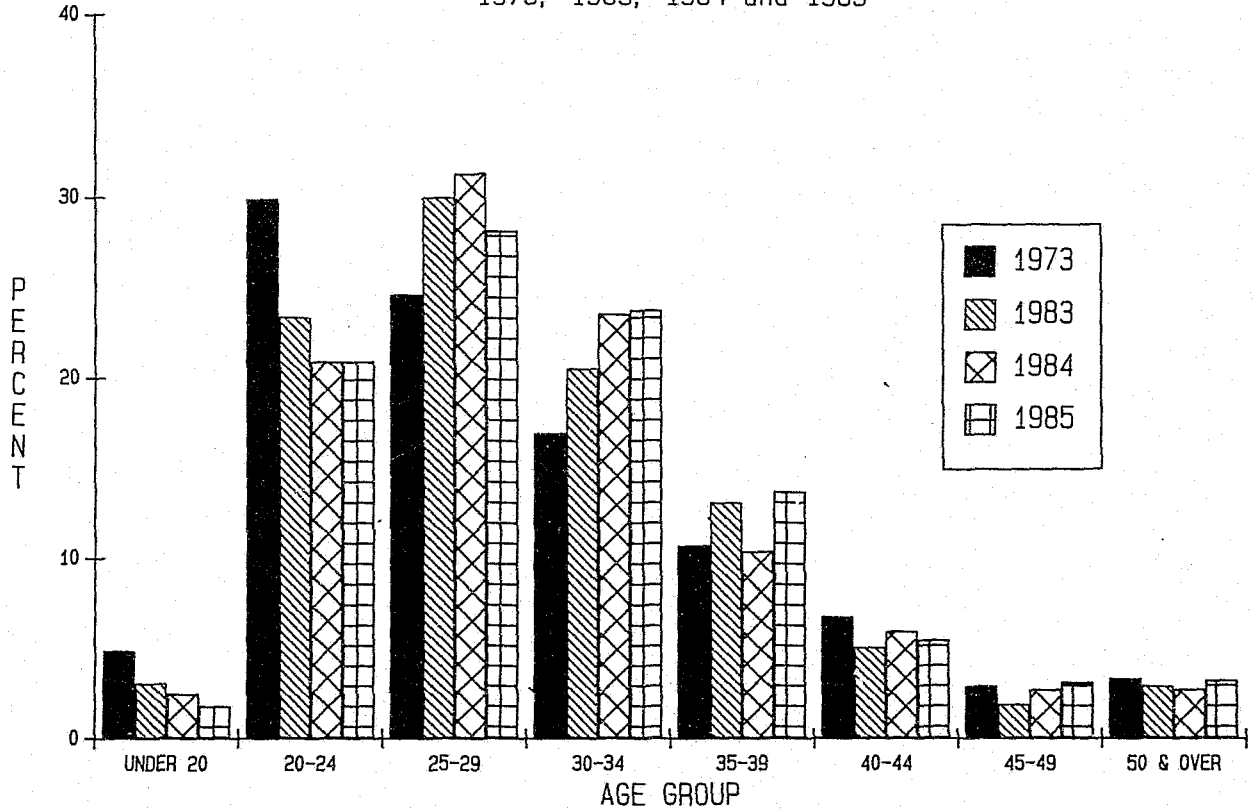
CHART III B AGE AT ADMISSION Female Felons Newly Received From Court 1973, 1983, 1984 and 1985
