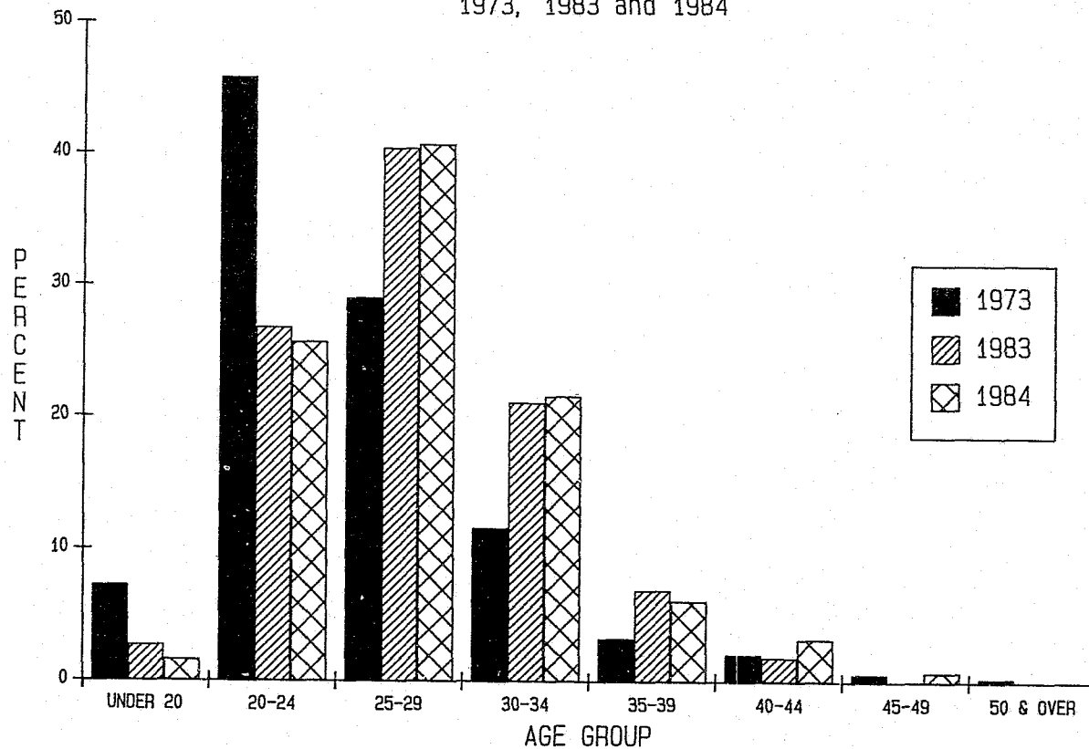
CHART XIV B AGE AT ADMISSION Female Civil Narcotic Addicts Newly Received From Court 1973, 1983 and 1984
