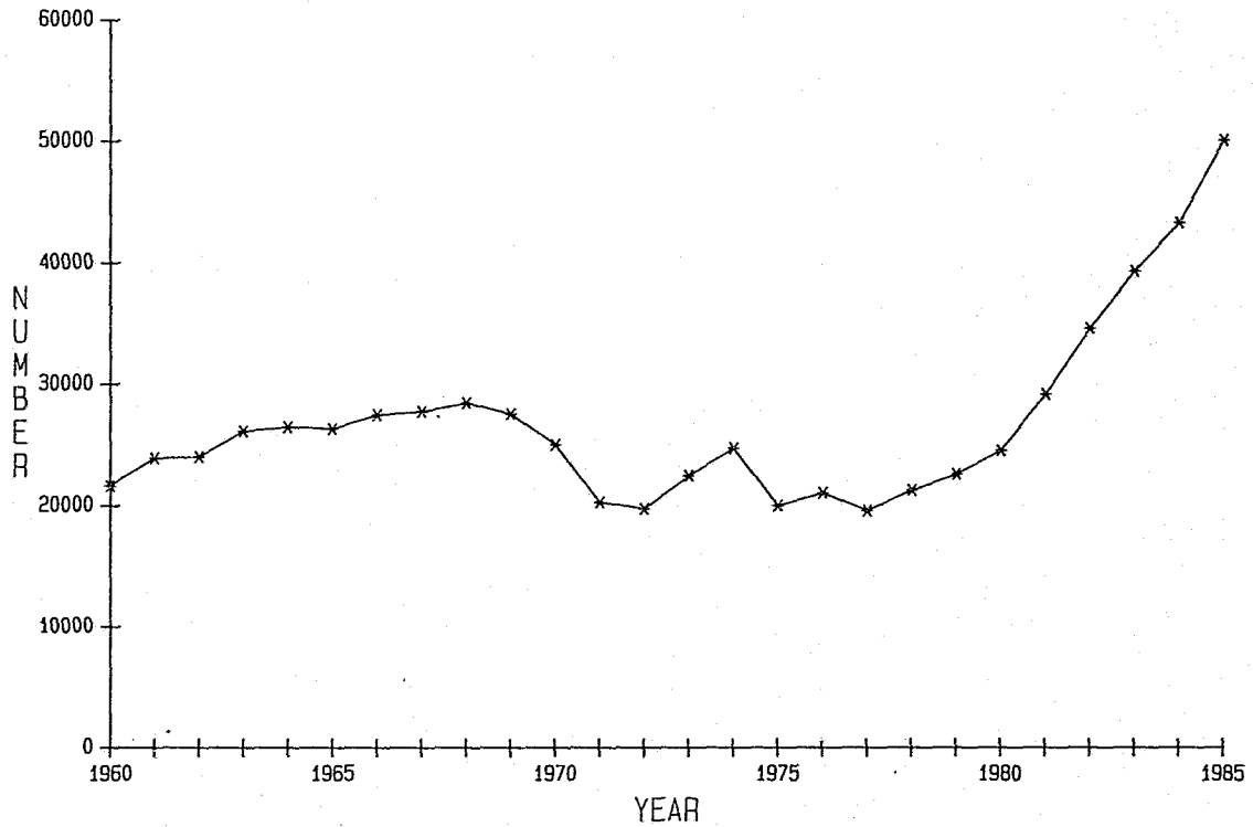
CHART I INSTITUTION POPULATION December 31, 1960 through 1985
