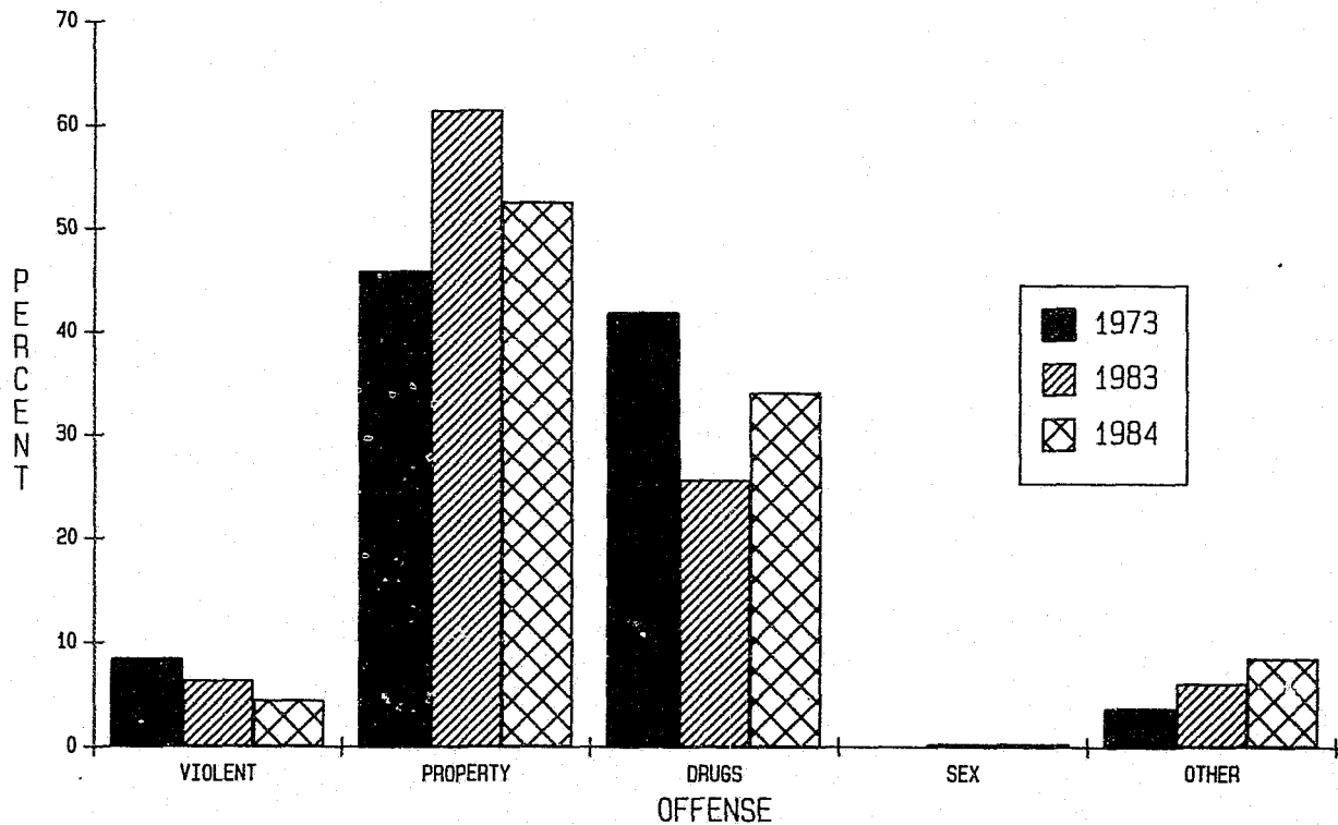
CHART XII A OFFENSE GROUPS Male Civil Narcotic Addicts Newly Received From Court December 31, 1973, 1983 and 1984
