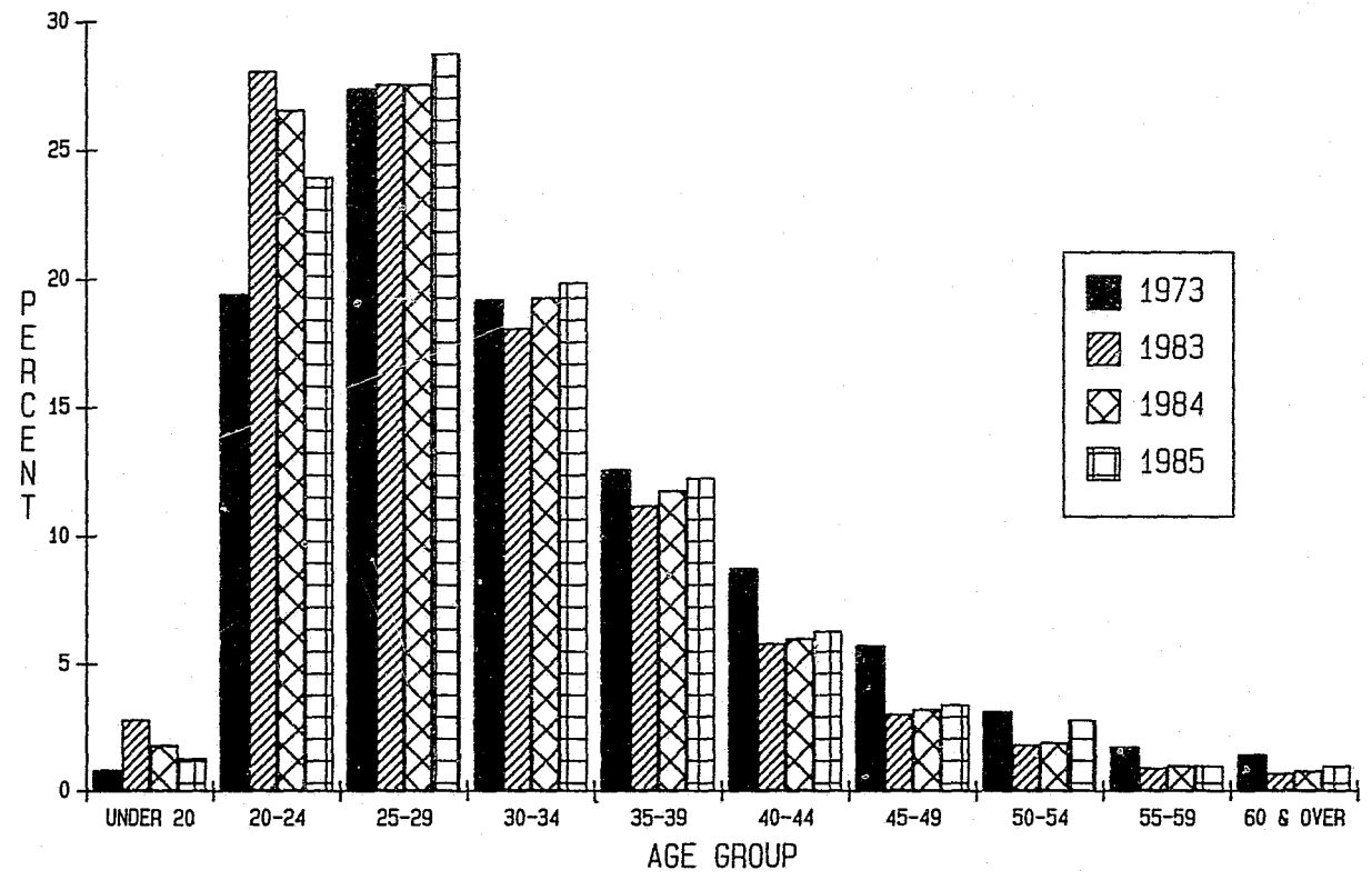
CHART VI A AGE GROUP Percentage Distribution of Male Felons in Prison December 31, 1973, 1983, 1984 and 1985
