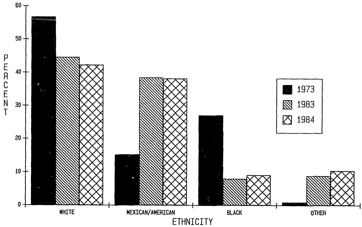
CHART XIII B RACIAL-ETHNIC GROUP Female Civil Narcotic Addicts Newly Received From Court 1973, 1983 and 1984
