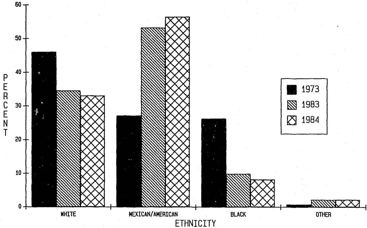
CHART XIII A RACIAL-ETHNIC GROUP Male Civil Narcotic Addicts Newly Received From Court 1973, 1983 and 1984
