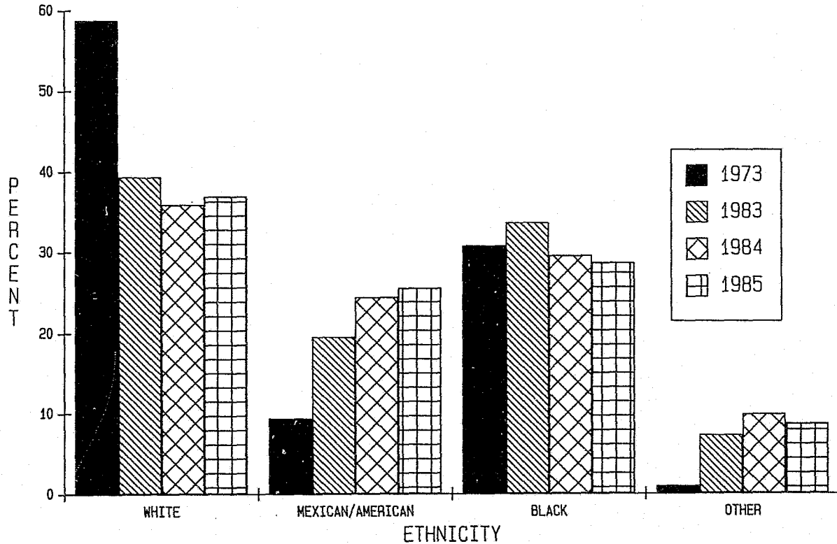
CHART IV B RACIAL-ETHNIC GROUP Female Felons Newly Received From Court 1973, 1983, 1984 and 1985
