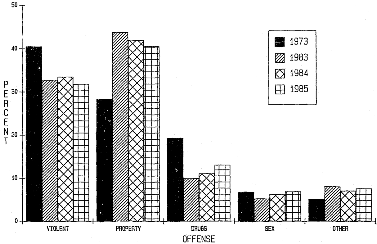
CHART XI A OFFENSE GROUPS Percentage Distribution of Male Felons on Parole December 31, 1973, 1983, 1984 and 1985
