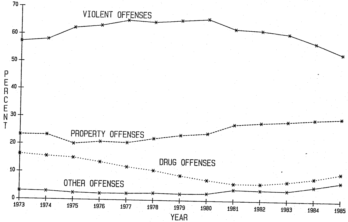
CHART V A OFFENSE GROUPS Percentage Distribution of Male Felons in Prison December 31, 1973 through 1985
